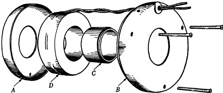
FIG. A-1.—Construction of simple focus coil. Focus coil and case. A , front half shell (0.062"); B , rear half shell (0.062"); C , center tubing, 1½ in. ID, 1¾ in. OD, with turned shoulder, to be peened into B ; D , coil, 1½ in. ID, 3½ in. OD, 1½ in. long.
