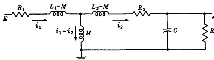
Fig. 10-15.—Equivalent circuit for a synchro.
