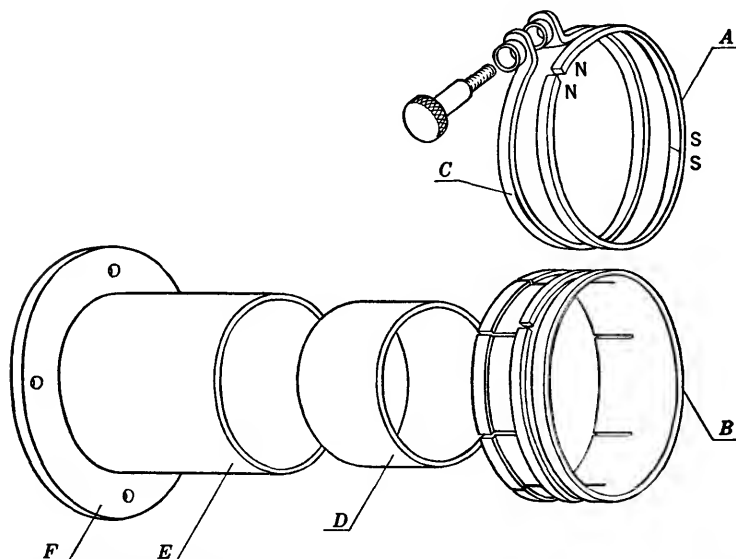
FIG. 9-5.—Precognizing assembly. A , the magnet—GE “Cunife” alloy 0.120 \times 0.050 strip, rolled into 2-in. ID circle; B , brass ring; C , brass clamping ring; D , soft iron shunt to be soldered into rear end of supporting cylinder; E , brass supporting cylinder; F , mounting flange.
