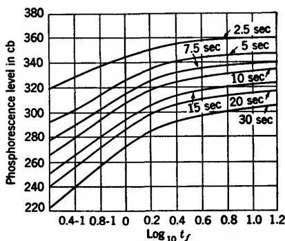
FIG. 18-23.—Change in phosphorescent levels after varying periods of raster excitation at 500 cb, observed at times indicated. Duration of excitation t_f in minutes.
