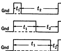
FIG. 4-8.—Level stabilization by d-c restoration.
