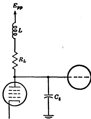
FIG. 4-60.—Shunt peaking.
