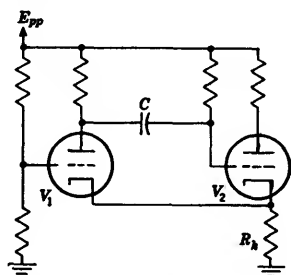
FIG. 4-26.—Cathode-coupled flip-flop circuit.
