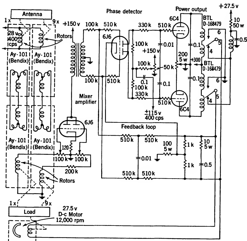
FIG. 5.9.—Airborne 400-cps relay servo.
