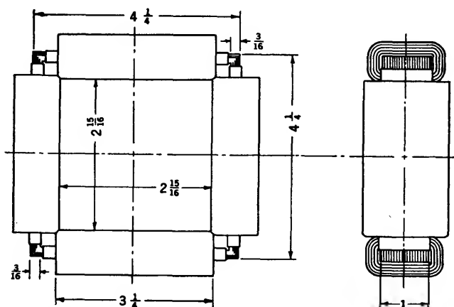
FIG. B-4.—Square iron-core off-centering coil. Core: Laminated silicon steel. Coils: Layer-wound, No. 28 enameled wire. Paper insulation between layers. First ten layers: 220 T/layer, 3-in. winding length; second ten layers: 200 T/layer, 2.9-in. winding length; last layer: 180 T/layer, 2.8-in. winding length. Total turns = 4380.
