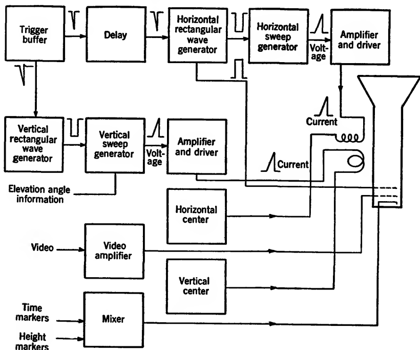
FIG. 15-5.—RHI block diagram.
