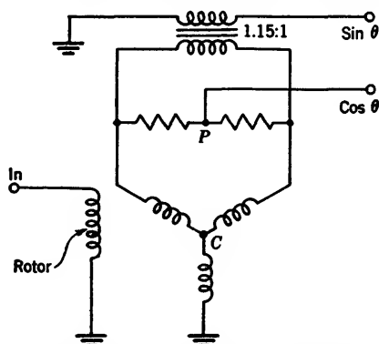
Fig. 5-30.—2-phase output from 3-phase synchro.
