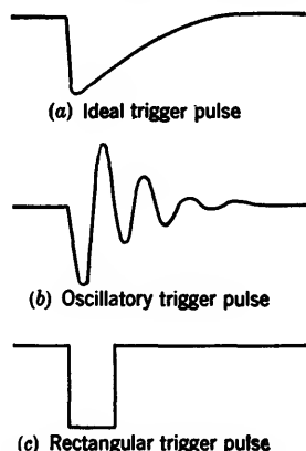
FIG. 4-17.—Typical trigger waveforms.
