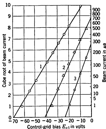
FIG. 2-27.—Static characteristics of three 5FP7 cathode-ray tubes at E_b = 4\text{kv} , E_{c2} = 250 volts.
