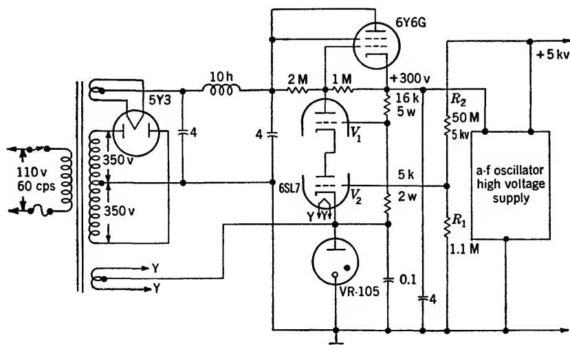
FIG. 4-85.—Voltage regulation with load feedback.
