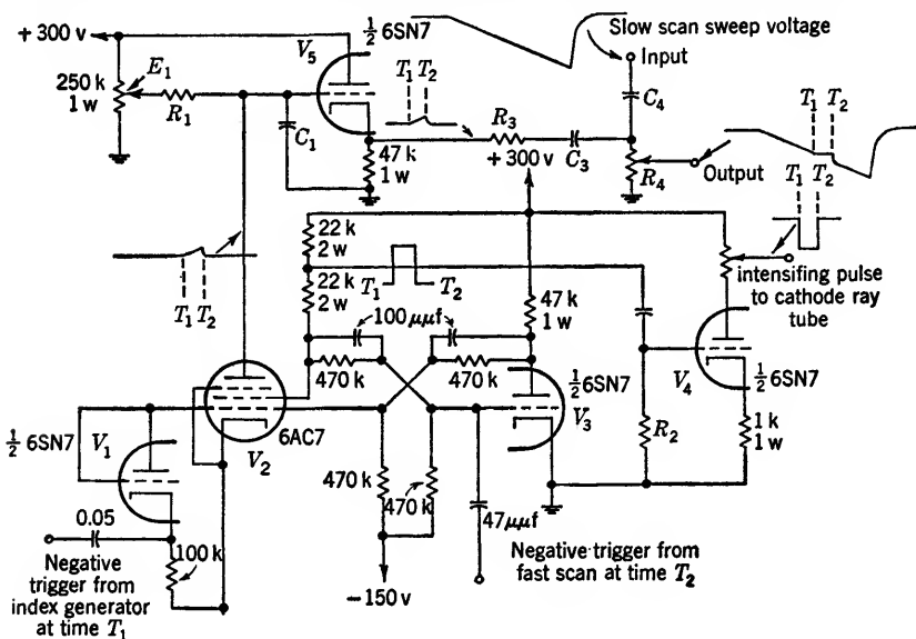
FIG. 6-8.—Sweep-stopping circuit.
