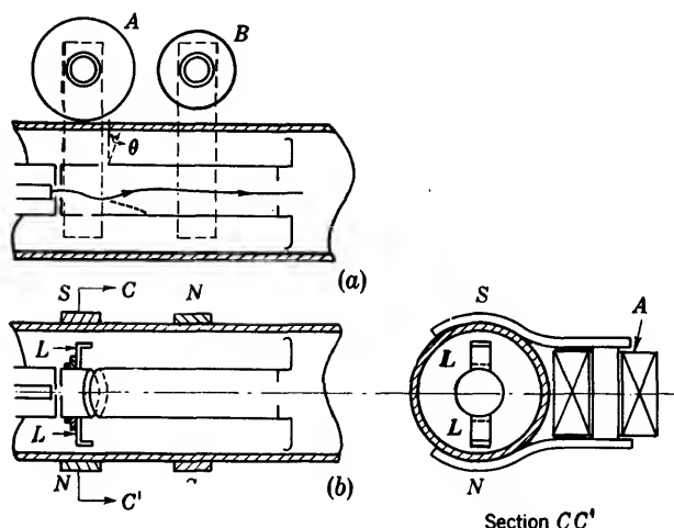
FIG. 2-36.—Ion-trap gun.
