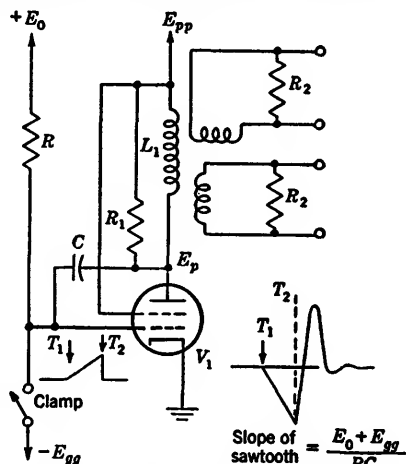
Fig. 10-17.—Miller-rundown sawtooth-voltage driving circuit for a synchro.
