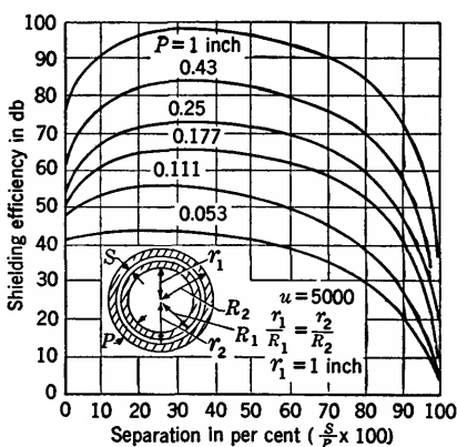
FIG. 16-15.—Shielding efficiency of two concentric cylinders vs. the air gap between them. The total thickness of the shield P is kept constant. (Courtesy of Bell System Technical Journal.)
