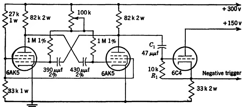
Fig. 4-21.—Multivibrator designed for maximum stability; 1600 cps.
