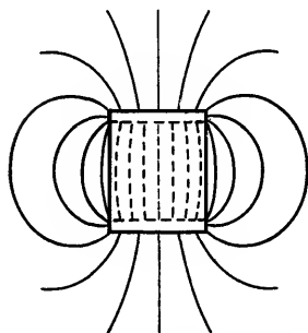
FIG. 8-8.—Axial magnetic-field distribution of a typical square iron-core coil.
