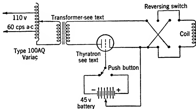
FIG. 12-8.—Magnetizing circuit.
