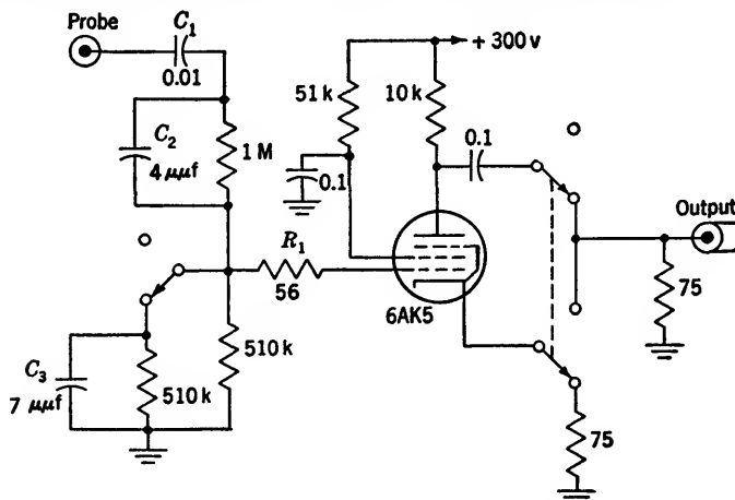
FIG. 7-12.—Video test probe, schematic diagram.
