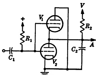
FIG. 4-34.—Two-way double-triode clamp.
