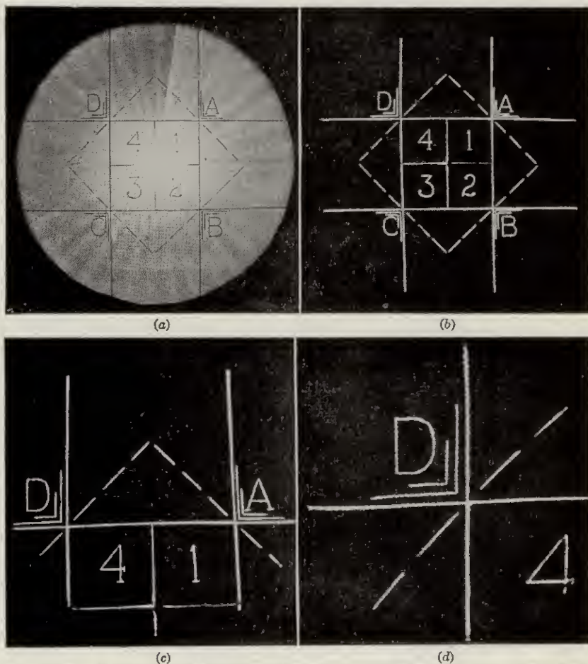
FIG. 16-24.—Photographs of a video-map transmitter CRT with a PPI scan (linear radial trace 1800 \mu\text{sec}/\text{radius} ) and of several receiving displays with the same type of scan.
