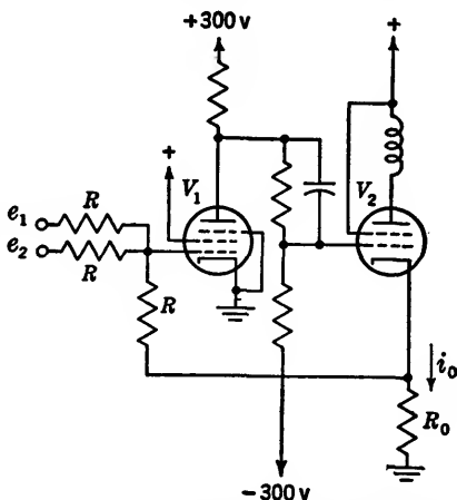
FIG. 10-12.—Direct-coupled feedback circuit for producing an output current i_0 proportional to e_1 + e_2 . R \gg R_0 .
