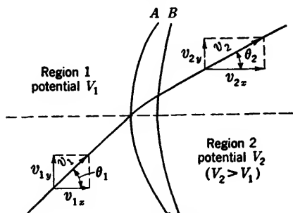
FIG. 2-2.—Refraction of electrons in an electric field.
