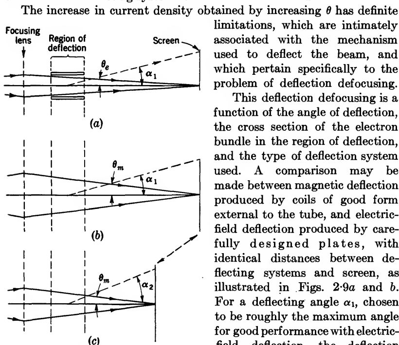
FIG. 2-9.—Comparison between deflection by electric and magnetic fields. (a) Deflection by electric field. (b) Deflection by magnetic field. (c) Shortened tube.
