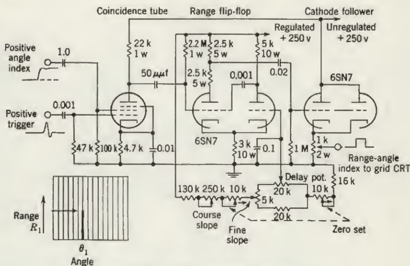
FIG. 6-16.—Range-angle index generator.
