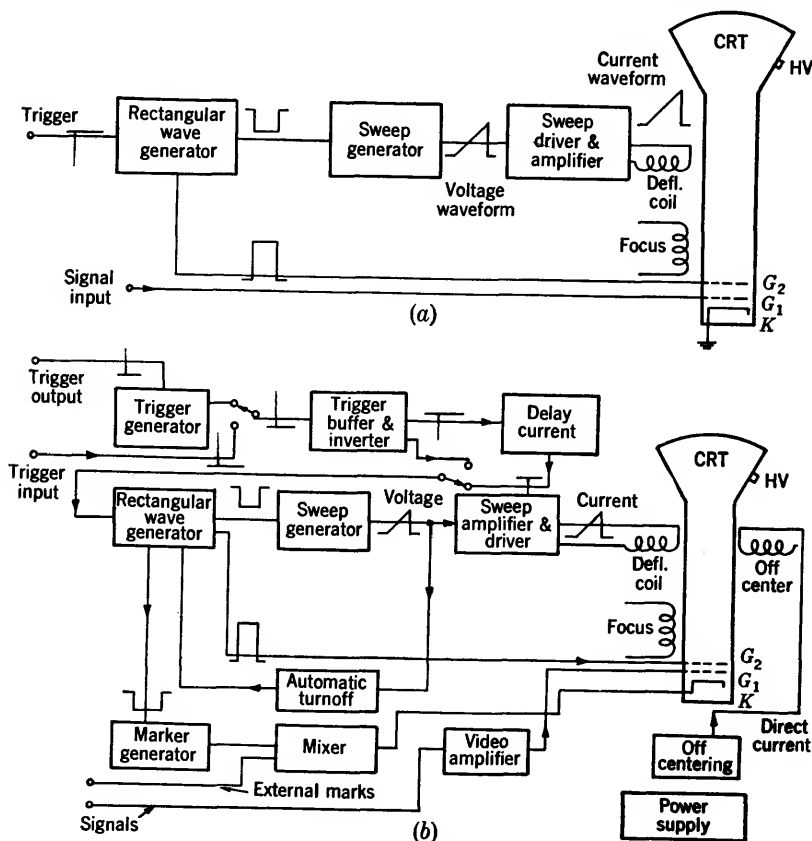
FIG. 13-1.—Block diagram of radial-time-base display.
