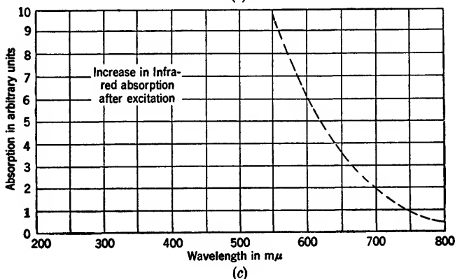
FIG. 18-5.—Absorption and emission curves for sulfide phosphors. (a) Relative absorption bands for zinc and cadmium sulfides. (b) Relative emission bands for zinc and sulfides. (c) Assumed increase in infrared absorption after electronic excitation of a long-persistent sulfide phosphor.
