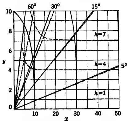
FIG. 15-2a.—Distortion due to approximations \cos \alpha = 1 and \sin \alpha = \alpha . — y = t \sin \alpha , x = t \cos \alpha ; lines of constant t and constant \alpha are shown; lines of constant height are horizontal. --- y = t\alpha , x = t ; lines of constant h and constant \alpha are shown; lines of constant t are vertical.
