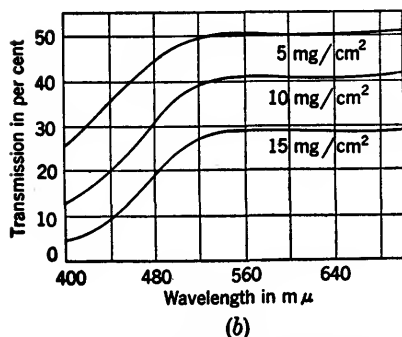
FIG. 18-8.—Spectral transmissivities of two phosphor types and three screen thicknesses. (a) (93)ZnS:(7)CdS:Cu. (b) (75)ZnS:(25)CdS:Cu.
