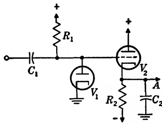
FIG. 4-33.—One-way diode-cathode-follower clamp.
