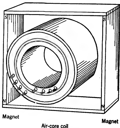
FIG. 12-1.—Permanent-magnet off-centering with external magnet.
