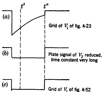
FIG. 4-51.—Grid waves of various flip-flop circuits.
