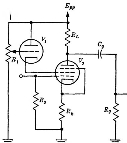
FIG. 4-61.—Gain controlled by screen voltage.
