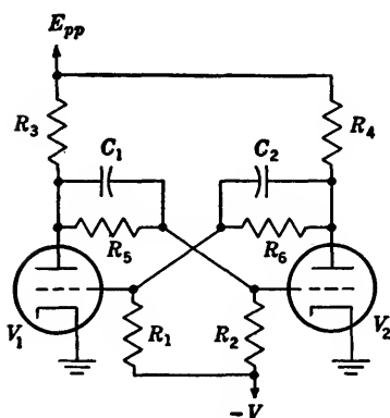
FIG. 4-24.—Scale-of-two circuit.
