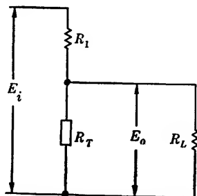
FIG. 4-74.—Nonlinear resistance regulator.
