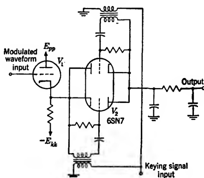
FIG. 5-16.—Keyed detector.
