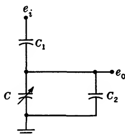
FIG. 5-35.—Condenser-divider network.
