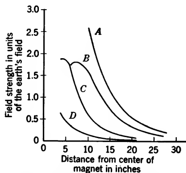
FIG. 3-22.—External field around a focus magnet with and without shielding.
