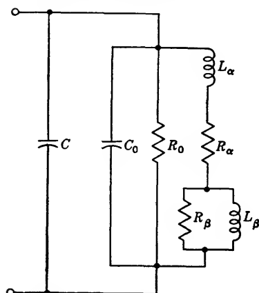
FIG. 8-23.—Connection for additional condenser across deflection coil.
