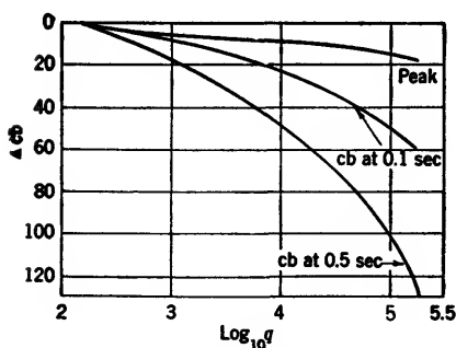
FIG. 18-29.—Change in radiance levels of \text{ZnF}_2\text{:Mn} phosphor following excitations repeated at the rate of 60 per second with charge density per excitation of 20 \text{ m}\mu\text{c}/\text{cm}^2 . Total q in microcoulombs per square centimeter.
