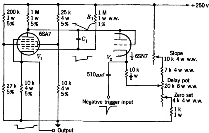
FIG. 6-11.—Phantatron delay circuit.
