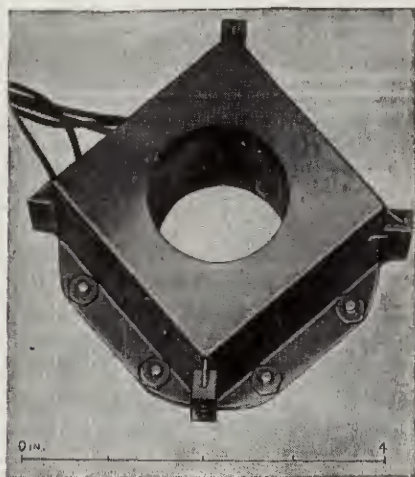
FIG. 8-15.—Copper shield for an iron-core deflection coil.
