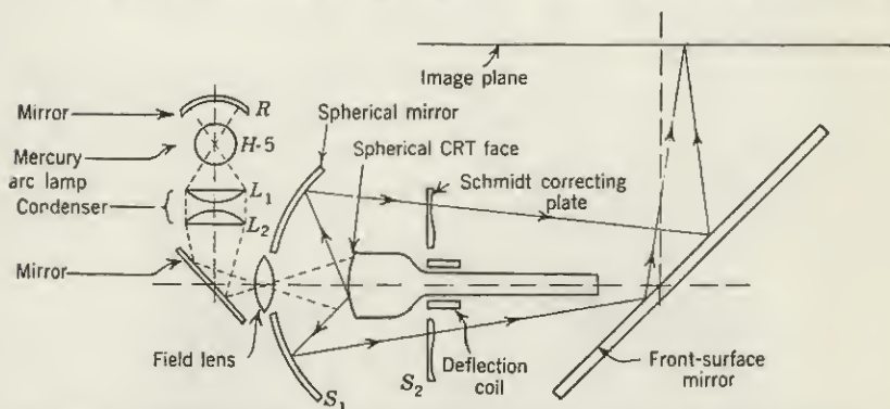
FIG. 16-30.—Projection and illumination optics used in dark-trace projection indicators.
