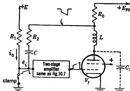
FIG. 10-9.—Three-stage feedback amplifier.
