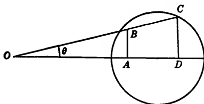
FIG. 14-15.—Sector display generation: two time bases. For any angle \theta , the sweep moves along AB in the time corresponding to the range OA ; then it moves along BC at the end of the time delay that gives OA . The line BC is the resultant of two motions, one in the direction AB , the other in the direction AD .
