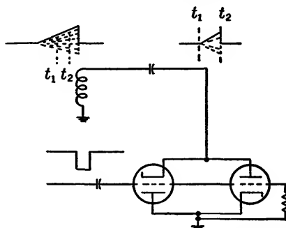
Fig. 14-21.—Method of deriving cosine-modulated sweep.
