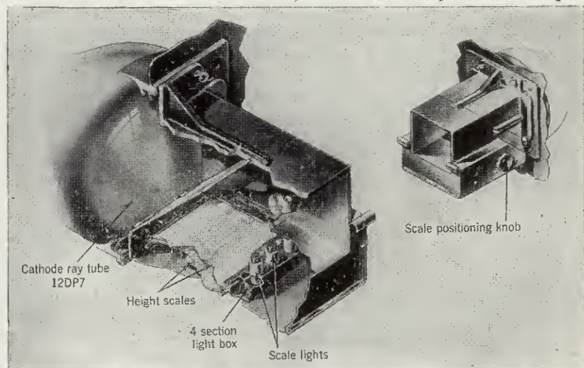
FIG. 16-19.—Height-indicator scale box, cut-away view.
