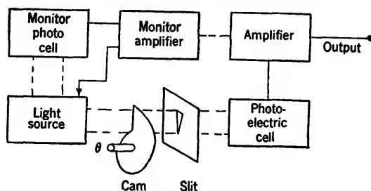
Fig. 5-42.—Electromechanical data-transmission system consisting of a cam and photoelectric cell.
