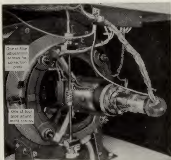
FIG. 16-32.—Detail of tube mount and drive.
