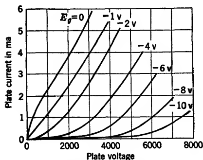
FIG. 4-77.—National Union M-1060 high-voltage triode characteristics.
