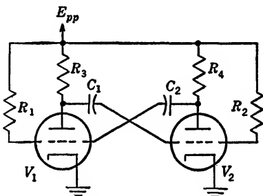
FIG. 4-22.—Multivibrator circuit.
