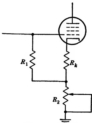
FIG. 4-62.—Gain controlled by cathode degeneration.
