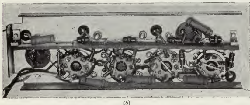
FIG. 7-6.—High-gain video circuit. (a) Circuit diagram. (b) Inside view.
