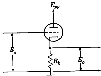
FIG. 4-10.—Cathode follower.
