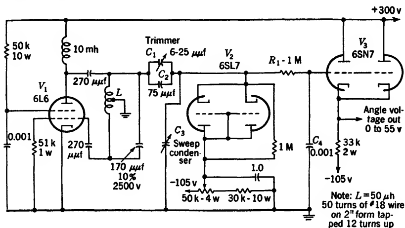
Fig. 5-37.—Angle-voltage generator.
