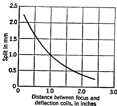
Fig. 9-9.—Line splitting for various focus-coil positions.
