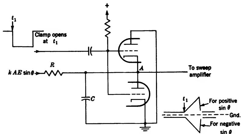
FIG. 13-27.—Sawtooth generator with two-way two-triode clamp.
