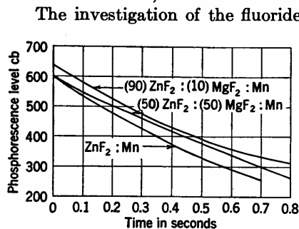
FIG. 18-28.—Phosphorescence of three fluorides as a function of time.
