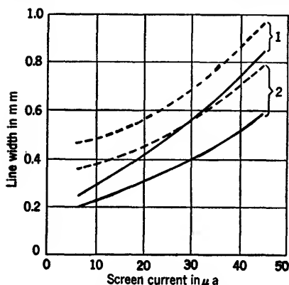
FIG. 2-19.—Typical line-width versus screen-current curves for 5CP1 cathode-ray tubes. Curves 1: E_{b2} = 1500 volts; E_{b3} = 3000 volts. Curves 2: E_{b2} = 2000 volts; E_{b3} = 4000 volts. Solid curve is measured at Position A, and dotted curve is measured at Position B.
