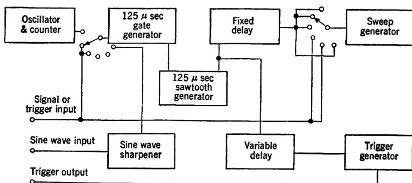
FIG. 7-7.—Block diagram of circuit operation.
