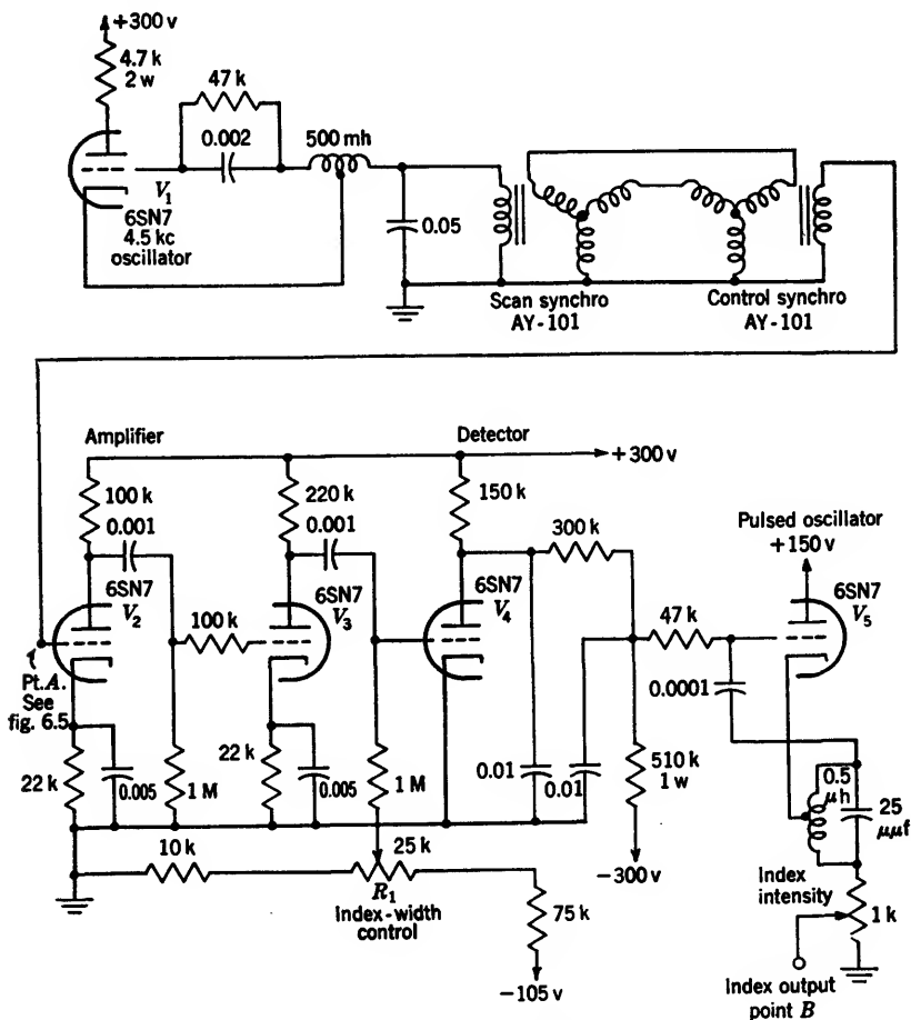
FIG. 6-4.—Synchro-null indices.
