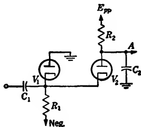
FIG. 4-32.—One-way double-diode clamp.
