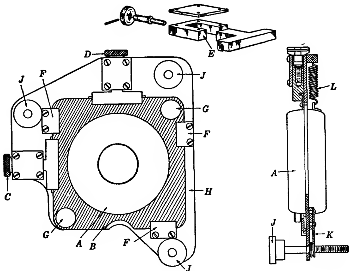
FIG. 3-15.—Adjustable support for focus coil. A, focus coil in case; B, sliding plate onto which focus coil is mounted; C, adjusting screw for horizontal motion of coil; D, adjusting screw for vertical motion of coil; E, detail of adjusting mechanism of C and D; F, retaining clamps for B; G, clamping screws for B; H, main plate; J, adjusting screws for tilting main plate to be threaded into fixed plate (not shown); K, spring clip support for J; L, tension spring (antibracklash).
