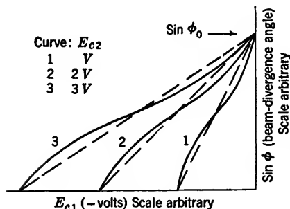
FIG. 2-8.—Relationship between grid drive and beam divergence.
