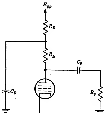
FIG. 4-58.—Plate decoupling used to compensate for droop produced by C_g R_g . R_D \ll R_g ; R_L \ll R_D ; C_D R_D = C_g R_g .
