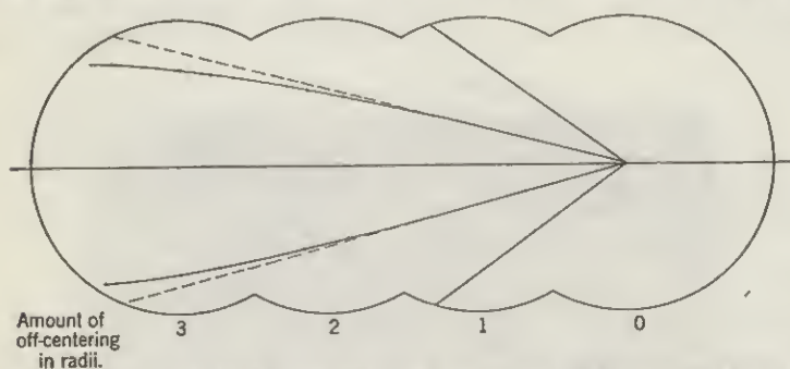
FIG. 12-13.—Composite showing traces for four conditions of off-centered radial sweep.
