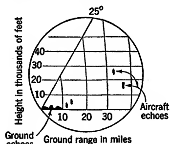
FIG. 1-5.—Range-height indication.
