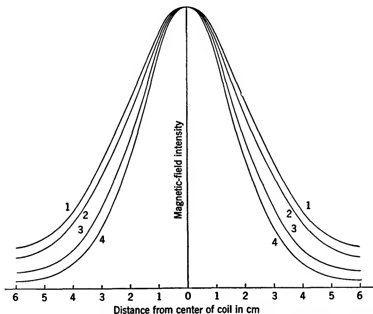
FIG. 8-16.—Axial field distribution of an iron-core coil with and without copper shield. 1. Coil without case. 2. With case—100 cps excitation. 3. With case—1000 cps excitation. 4. With case—10,000 cps excitation.
