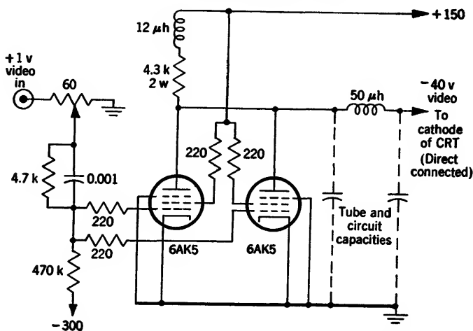
FIG. E-3.—Low-capacity tubes mounted at cathode-ray tube.
