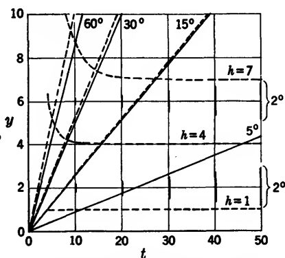
FIG. 15-2b.—Comparison of \sin \alpha and \alpha as elevation input information. --- y = t\alpha , x = t ; lines of constant h and \alpha are shown. — y = t \sin \alpha , x = t ; lines of constant \alpha are shown; lines of constant h are horizontal; the height of a 2^\circ signal is shown at various values of t .
