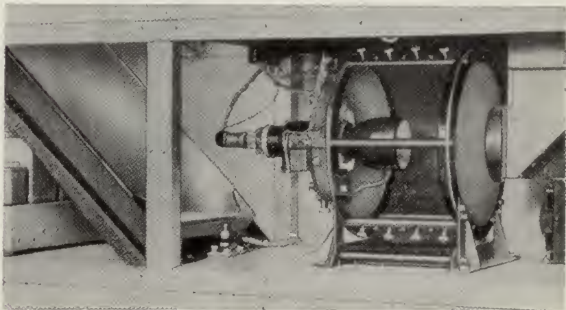
FIG. 16-31.—Side view of illumination and projection system.
