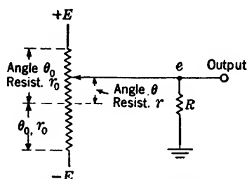
FIG. 5-27.—Use of a linear potentiometer to obtain an output voltage approximating the tangent function.
