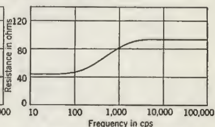
FIG. 8-19.—Variation of resistance of a typical iron-core deflection coil.
