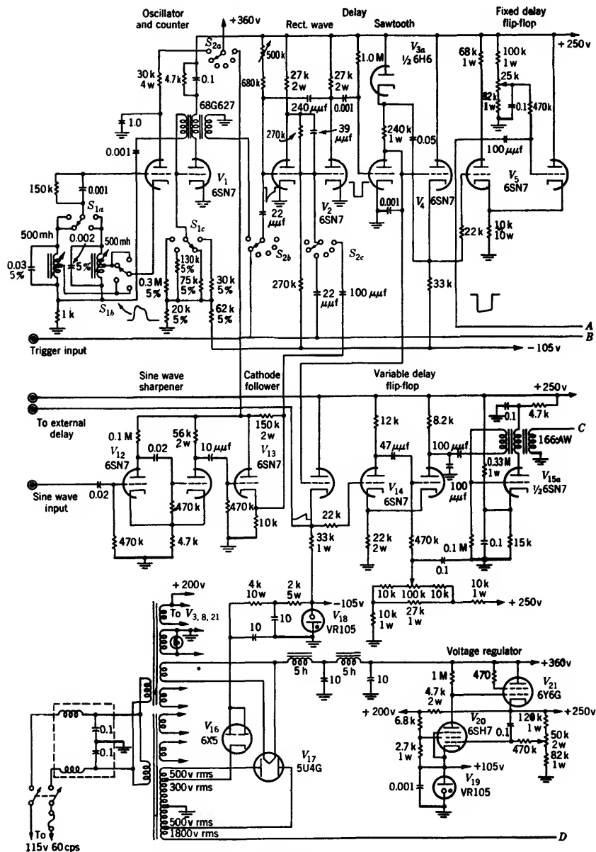
FIG. 7-8a.—Schematic circuit diagram of Model 5 synchroscope.
