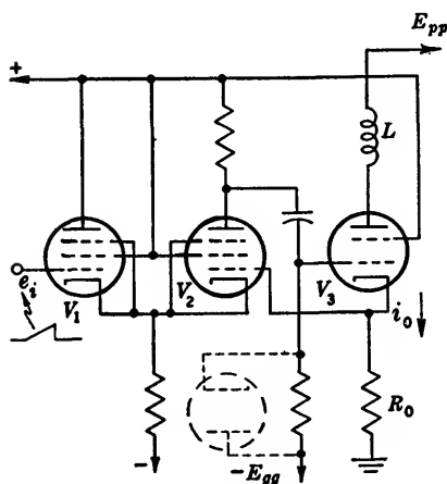
FIG. 10-10.—Another variety of feedback amplifier that causes a current waveform of the same shape as e_i to flow through the deflection coil.
