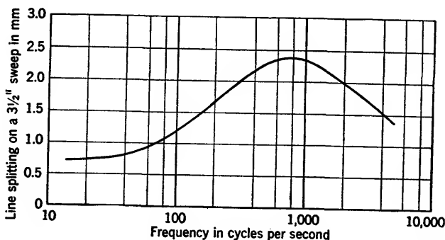
Fig. 9-8.—Line splitting vs. frequency with an iron case around the focus coil, and 0.15 in. between coils.
