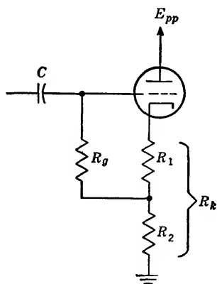
FIG. 4-14.—Method of increasing effective input resistance.
