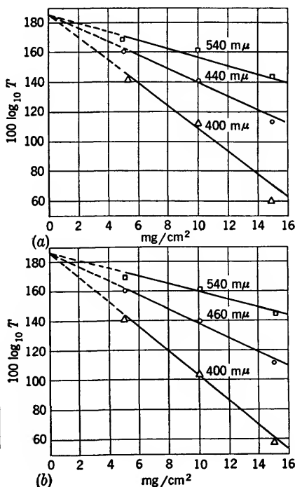
FIG. 18-9.—Plots to determine absorption coefficients at wavelengths shown for two screen materials. T is the transmission in per cent. (a) (93)ZnS:(7)CdS:Cu. (b) (75)ZnS:(25)CdS:Cu.
