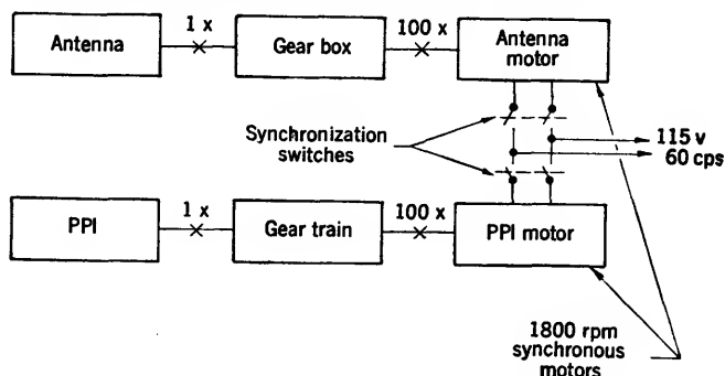
Fig. 5-43.—Synchronized data transmission with synchronous motors.
