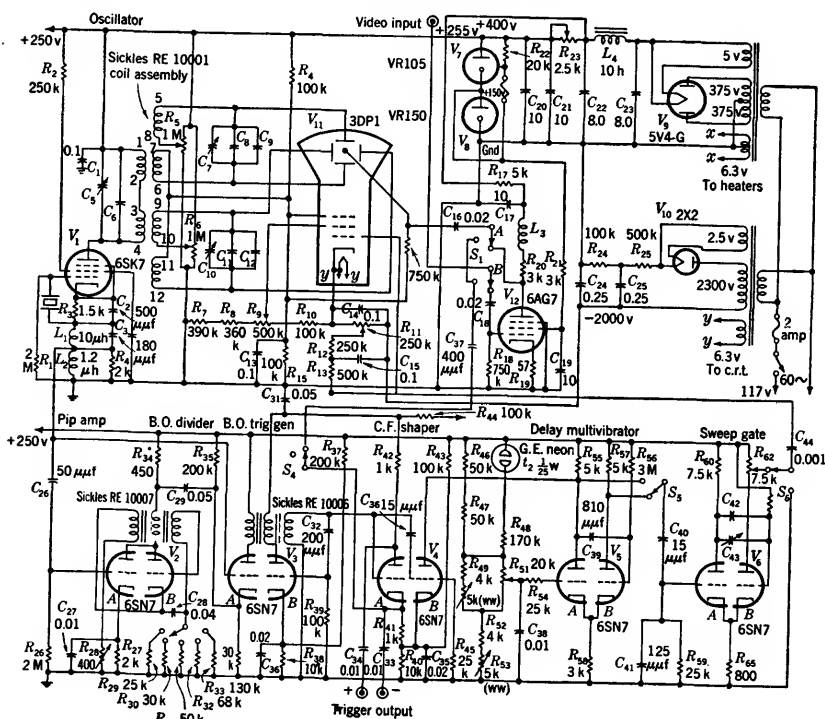
FIG. 7-28.—Model III range calibrator.
