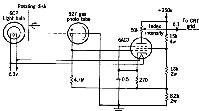
FIG. 6-3.—Photocell index circuit.
