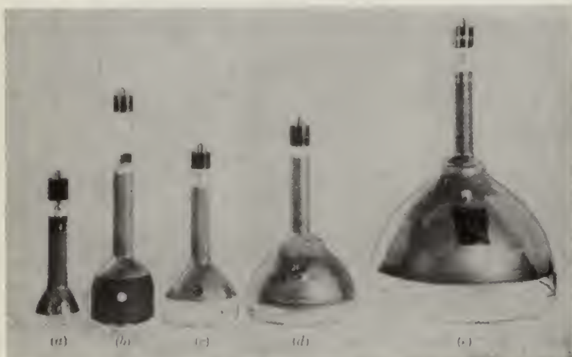
FIG. 2-25.—Typical magnetic cathode-ray tubes. (a) 3HP7; (b) 4AP10; (c) 5FP7; (d) 7BP7; (e) 12DP7.
