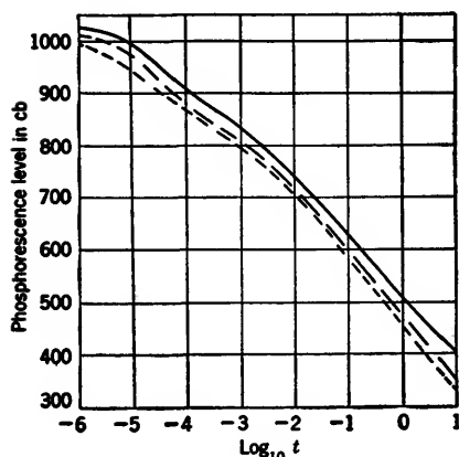
FIG. 18-25.—Phosphorescent decay following single pulse excitation and current density of j = 4 \text{ ma/cm}^2 . Time t in seconds. Excitation period 30 \mu\text{sec} —; 50 \mu\text{sec} ---; 200 \mu\text{sec} — · —. Screen type: (88)ZnS:(12)-CdS:Cu.
