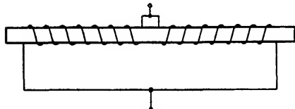
FIG. 8-12.—Balanced winding.
