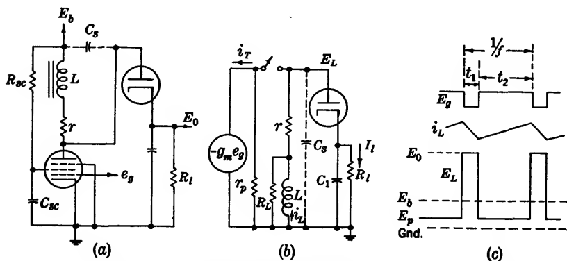
Fig. 4-84.—Inductance-charging generator. (a) Complete circuit. (b) Equivalent circuit. (c) Idealized waveforms.
