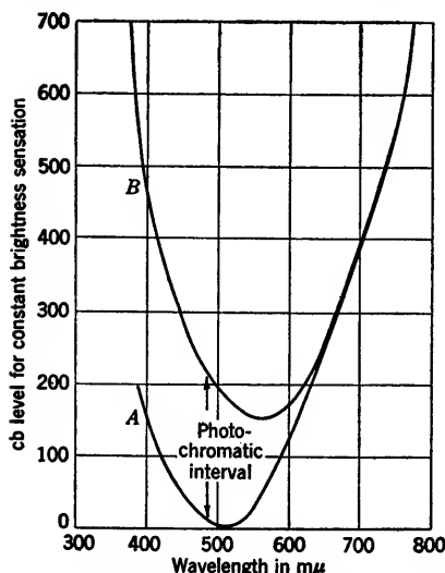
FIG. 18-46.—Relative spectral power levels for constant brightness sensation. Curve A—scotopic vision (dark-adapted eye); Curve B—photopic vision (I.C.I. standard luminosity curve), approximate threshold of cone vision.
