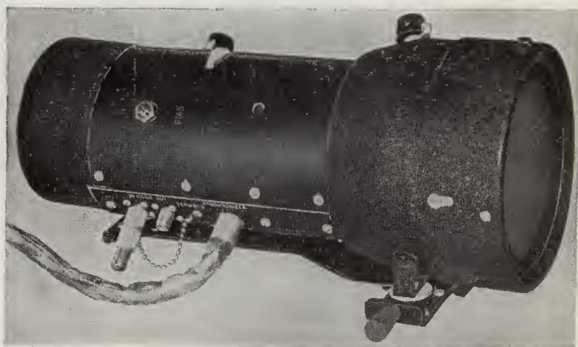
FIG. 16-5.—Fixed-coil mount for 5-in. magnetic tube, with permanent-magnet focusing and including amplifier. Top figure shows unit exposed.
