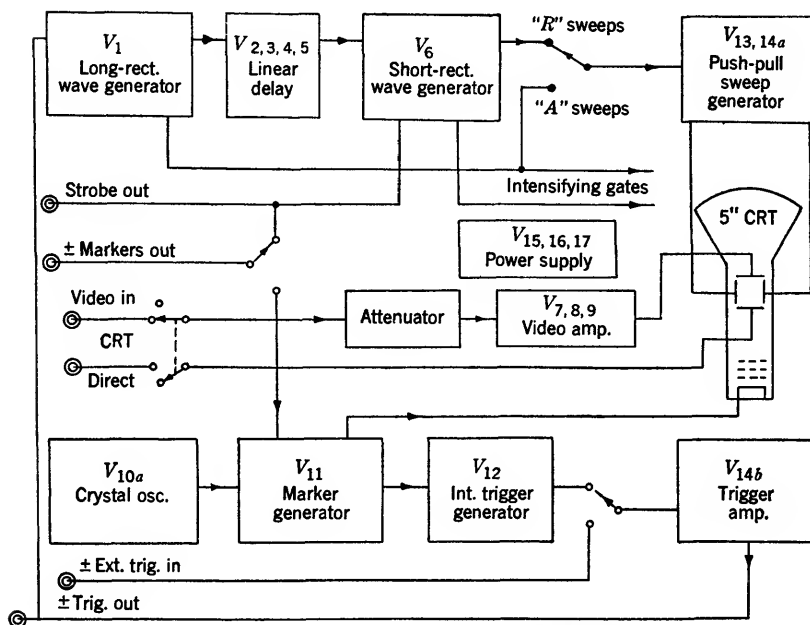
FIG. 7-16.—Block diagram of A/R range units Model 3.
