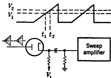
FIG. 14.25.—Diode pickoff circuit.
