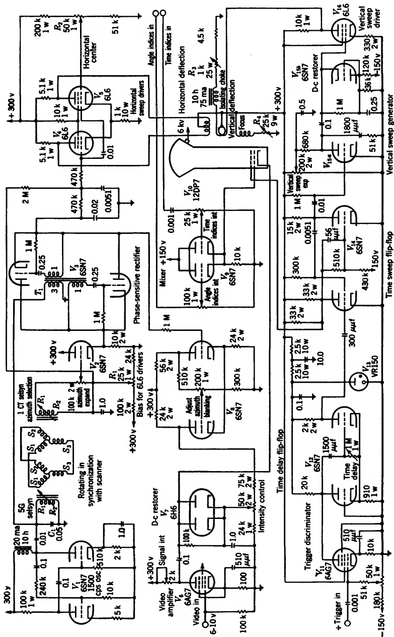
Fig. 11-7.—Circuit diagram, B-scan.
