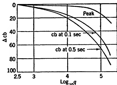
FIG. 18-30.—Change in radiance levels of (50)\text{ZnF}_2\text{:}(50)\text{MgF}_2\text{:Mn} phosphor following excitations repeated at a rate of 60 per second, with charge density per excitation of 20 \text{ m}\mu\text{c}/\text{cm}^2 . Total q in microcoulombs per square centimeter.
