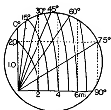
(b) Stretched PPI, 2 mile grid. Signals not shown
