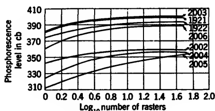
FIG. 18-14.—Buildup under repeated electron excitation. Screen excited at 10-sec intervals, with observation 1 sec after excitation. Q = 20 \text{ m}\mu\text{c}/\text{cm}^2 per raster. See Table 18-1 for screen compositions.
