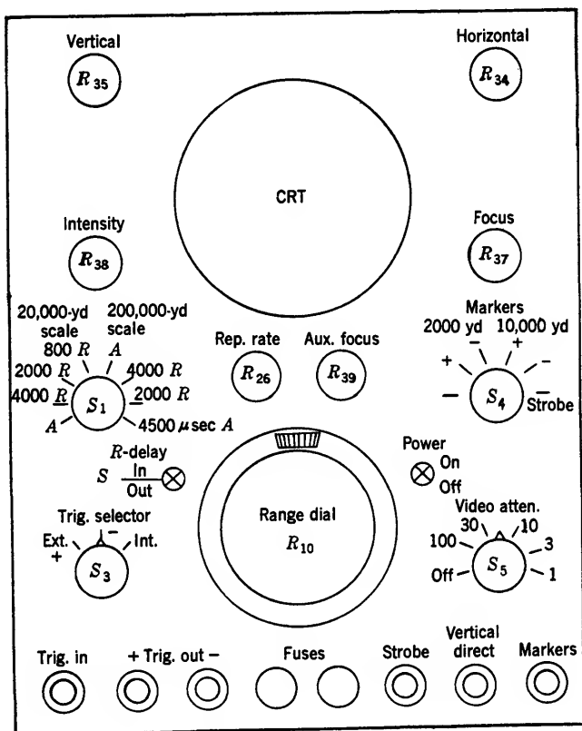
Fig. 7-20.—A/R-scope front-panel controls.
