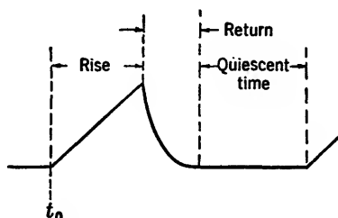
FIG. 4-37.—Sawtooth waveform.
