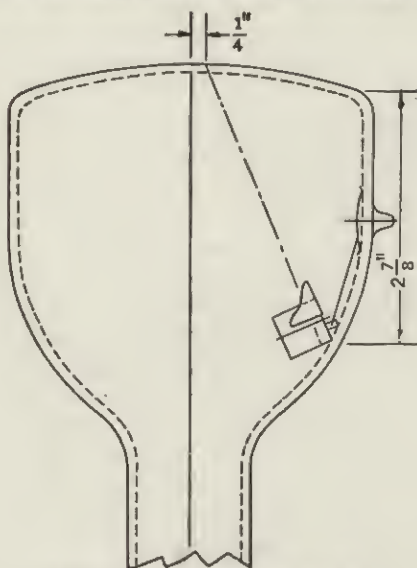
FIG. 18-65 —Evaporator mounting.
