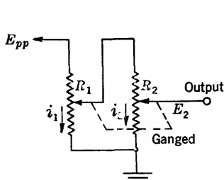
FIG. 5-23.—A means of obtaining an output voltage proportional to the square of a shaft rotation with a dual linear potentiometer. If R_2 \gg R_1 , i_1 = \frac{E_{pp}}{R_1} and i_2 = \frac{E_1}{R_2} .
