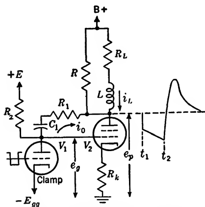
FIG. 10-4.—Voltage feedback for driving a deflection coil.
