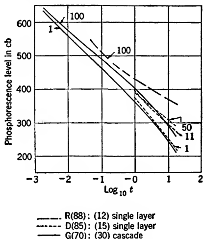
FIG. 18-40.—Comparison of phosphorescent decay from selected cascade and single layer screens. Time t in seconds.
