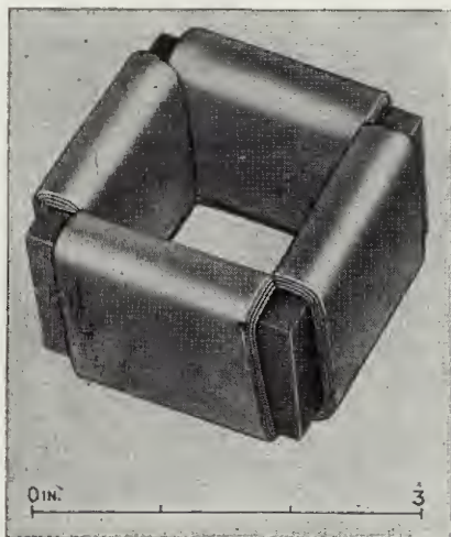
FIG. 8-11.—Iron-core deflection coil with two sets of windings.
