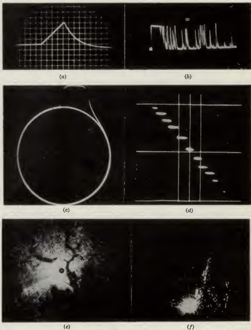
FIG. 1-3.—Typical cathode-ray tube displays.
