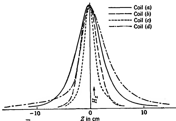
FIG. 3-2.—Intensity of axial component of focus field along axis for focus coils shown in Fig. 3-1.
