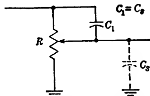
FIG. 4-65.—Compensated potentiometer.
