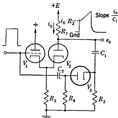
FIG. 10-5.—Circuit for generating a waveform e_o which has the approximate shape required to produce a linear current in an inductive load.
