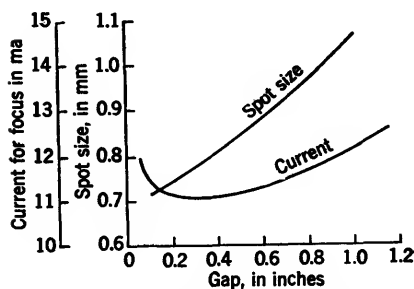
FIG. 3-3.—Spot size and focus current for various focus-coil gap widths; average for seven 7BP7 tubes; E_b = 5\text{ kv} ; I_b = 250\text{ }\mu\text{a} .
