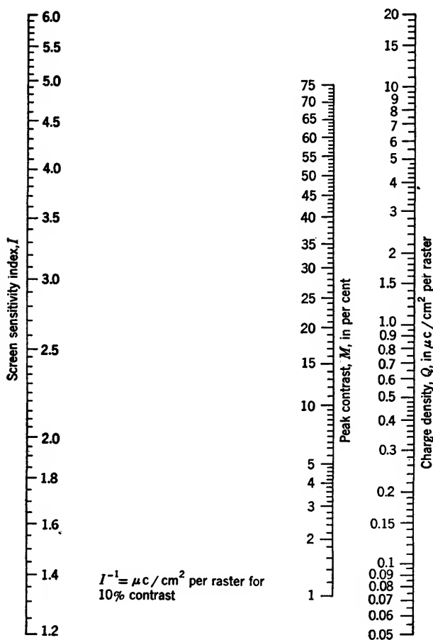
FIG. 18-51.— QM nomograph.
