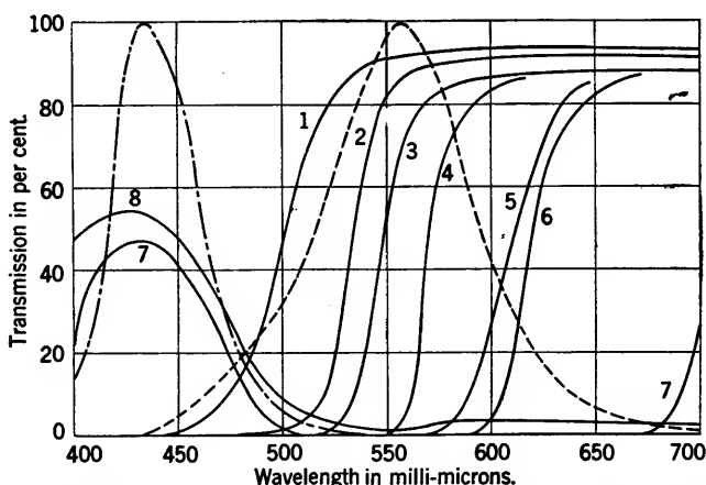
FIG. 16-17.—Transmission of various plastic filters. Curve 1, Plexiglas No. 106; Curve 2, Lucite No. H-10016; Curve 3, Plexiglas No. 121; Curve 4, Plexiglas No. 108; Curve 5, Plexiglas No. 159; Curve 6, Polaroid XDA8FAP; Curve 7, Polaroid X815 (0.003 in.); Curve 8, Monsanto A74592TVA (0.125 in.)
