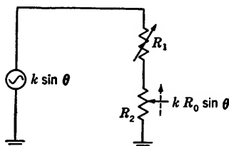
FIG. 14-7.—Range-normalization network.
