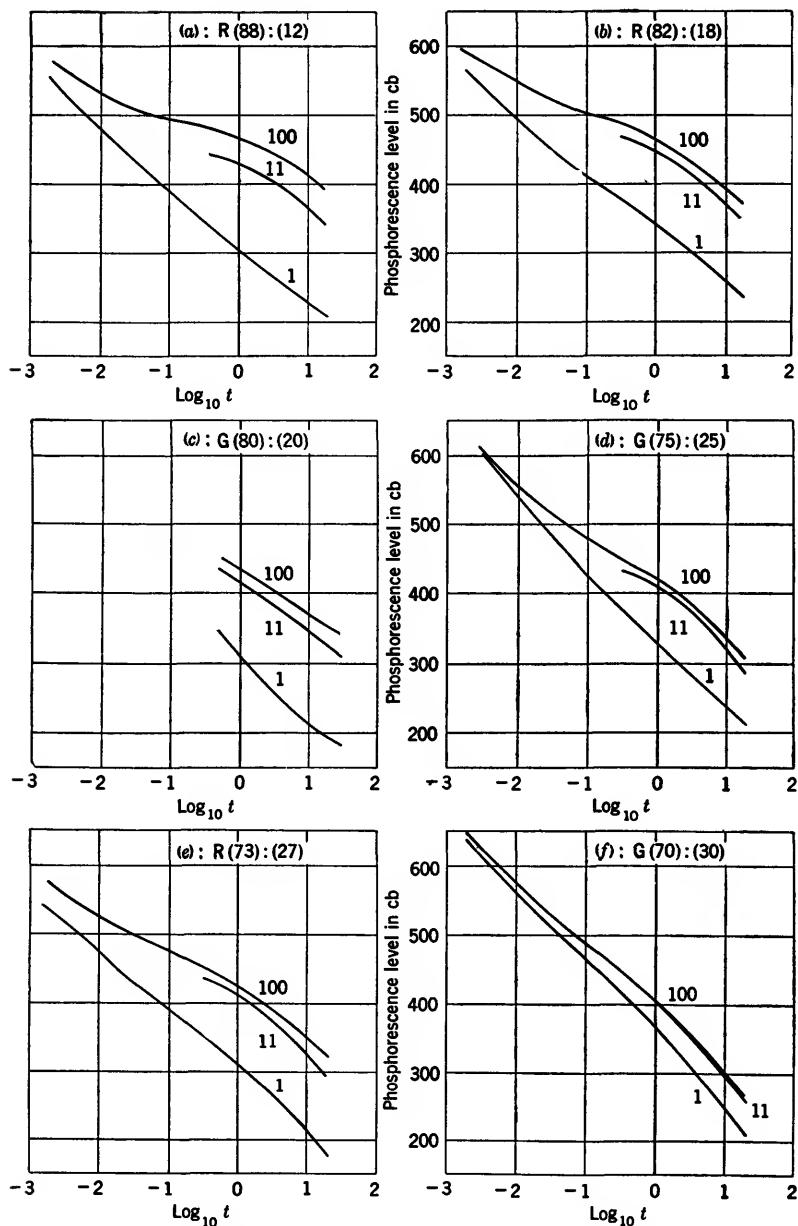
FIG. 18-39.—Phosphorescent decay for six different cascade screens. Excitation: 1, 11, and 100 rasters. 1-sec interval. Q = 20 \text{ m}\mu\text{c}/\text{cm}^2 , per raster. V_a = 4000 volts. Time t in seconds.
