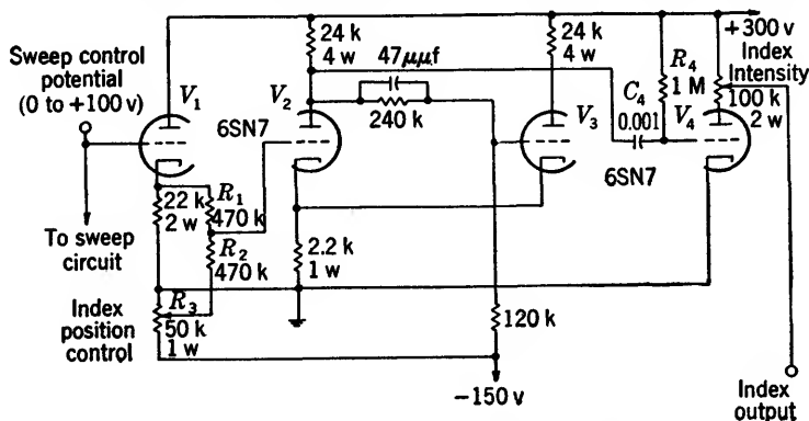
FIG. 6-6.—Index from sweep-control potential.
