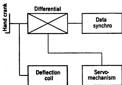
FIG. 14-8.—Mechanical schematic diagram for Micro-B scope. Hand crank turns deflection coil directly and phases data from data synchro. Servomechanism gives out control-data information of shaft motion.
