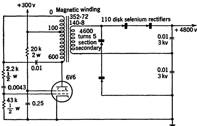
Fig. 4-80.—Audio-frequency voltage supply at 5 kc.
