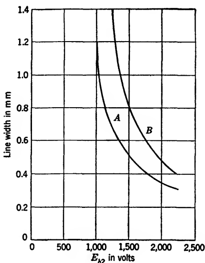
FIG. 2-18.—Variation of line width with anode voltage. Curve A: light output adjusted to 5 foot-lamberts. Curve B: light output adjusted to 10 foot-lamberts.
