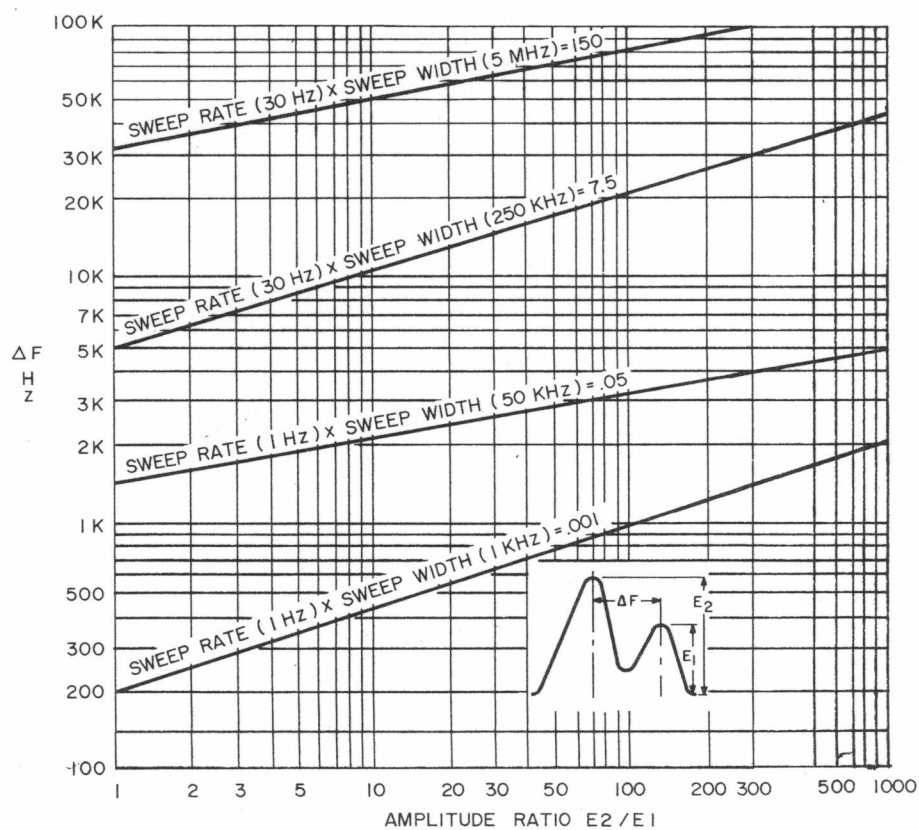
Figure 1-3. Typical Minimum Frequency Separation Required to Measure Amplitude Ratios (Skirt Selectivity)
