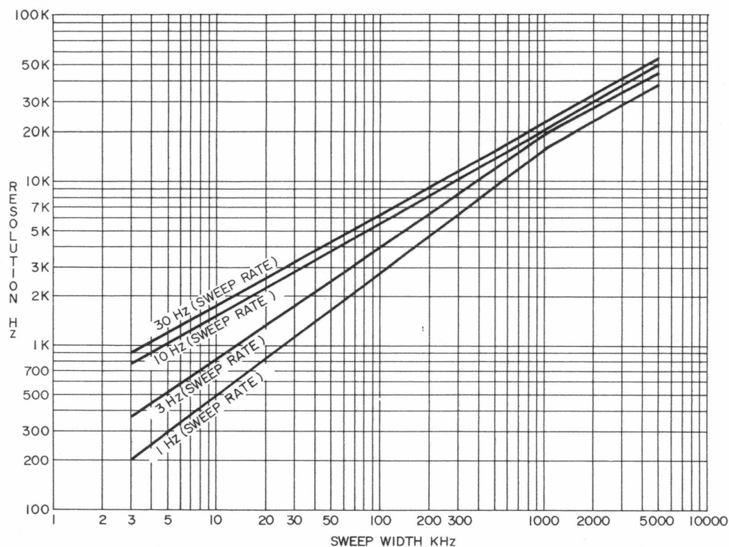
Figure 1-2. Typical Resolution Versus Sweep Width
