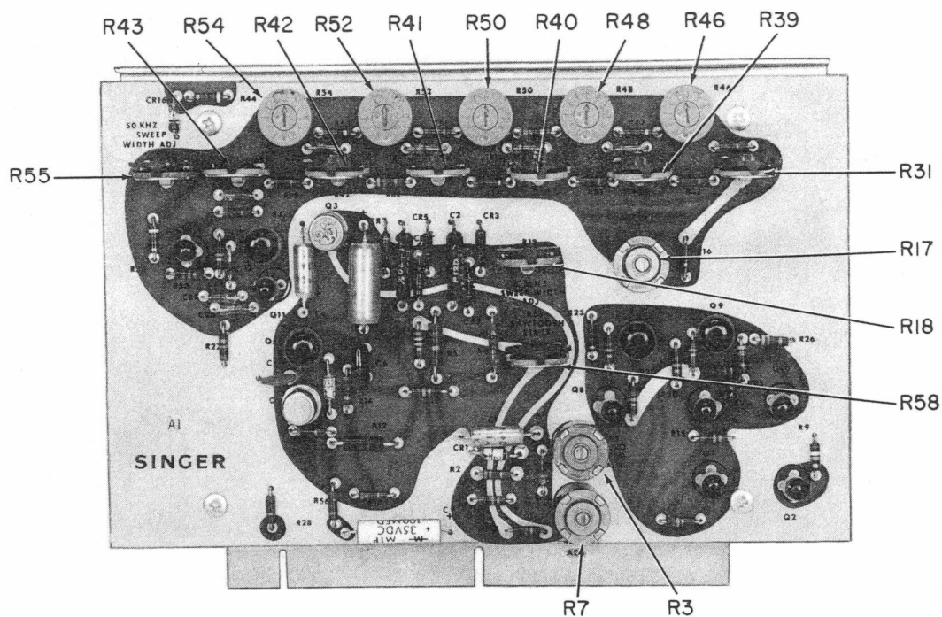
Figure 4-4. DC Control Module A1, Adjustment Locations
