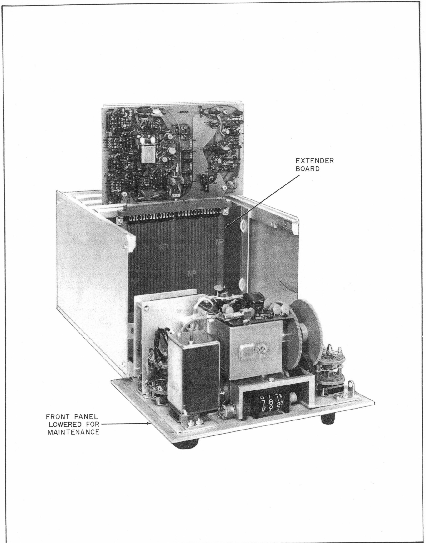
Figure 4-1. Extender Board
