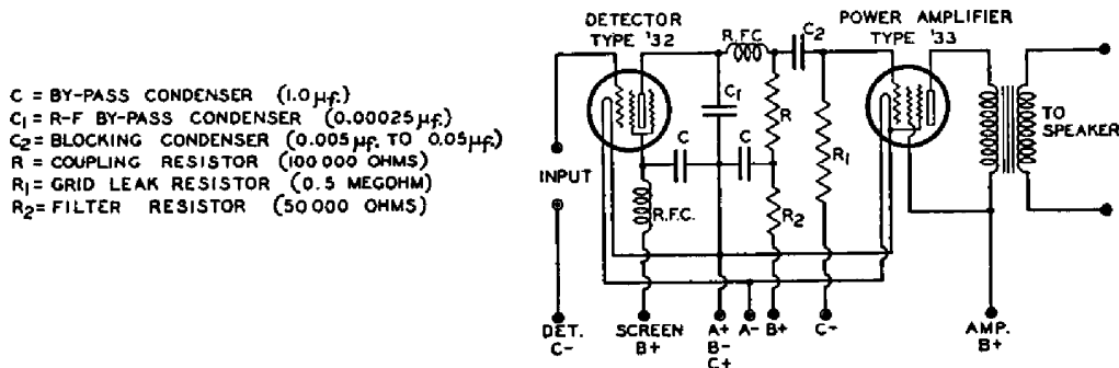
OPTIONAL DETECTOR AND AMPLIFIER—2-VOLT FILAMENT TYPES
