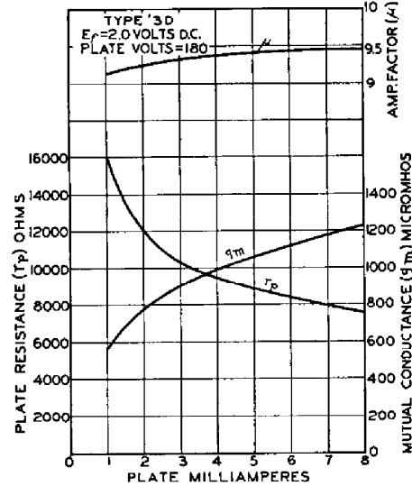
AVERAGE PLATE CHARACTERISTICS
