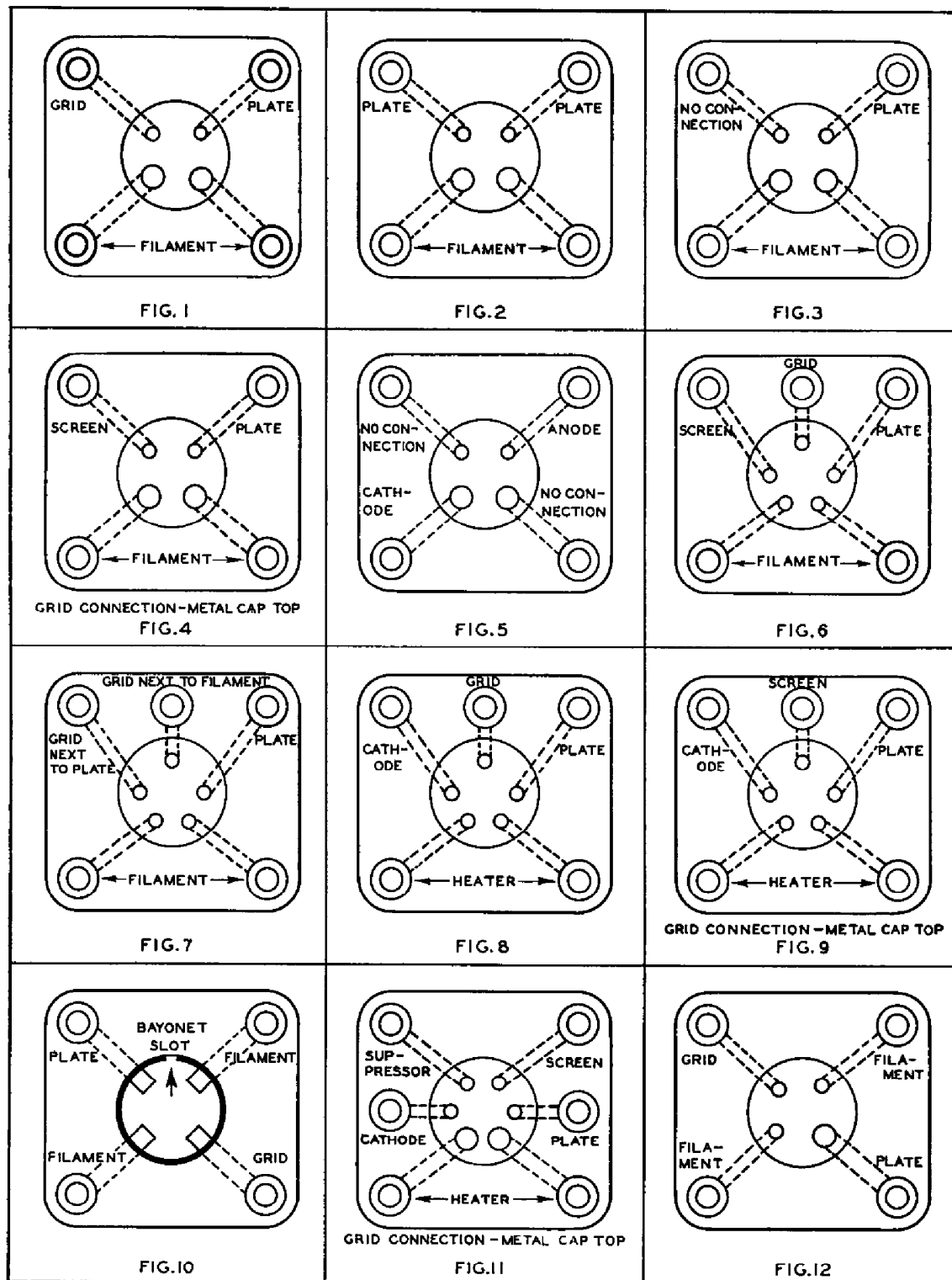
TOP VIEWS OF SOCKETS
