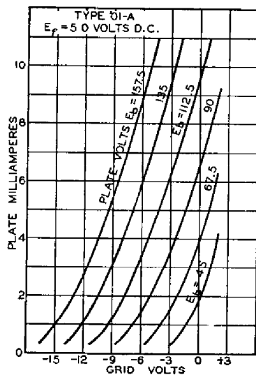
AVERAGE PLATE CHARACTERISTICS
