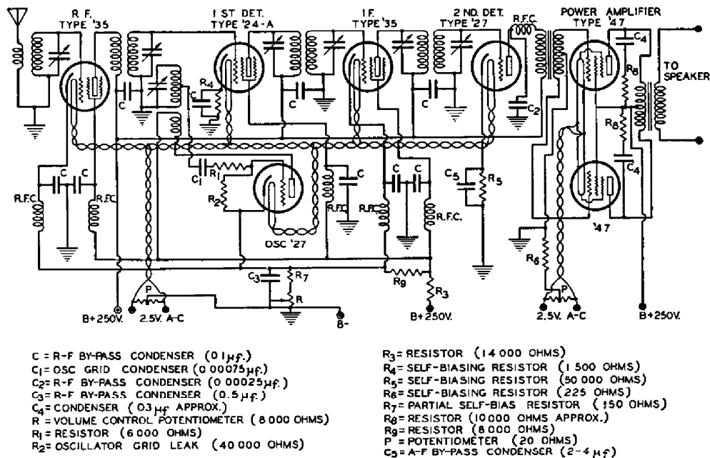
TYPICAL SUPERHETERODYNE RECEIVER FOR A-C OPERATION
