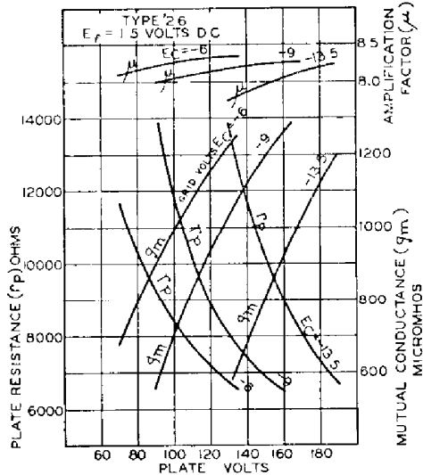
AVERAGE CHARACTERISTICS
