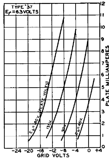
AVERAGE CHARACTERISTICS
