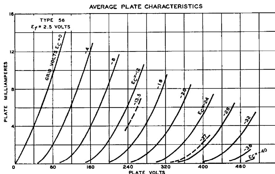
HIGH-GAIN AUDIO-FREQUENCY AMPLIFIER
