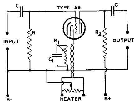
RESISTANCE-COUPLED A-F AMPLIFIER
