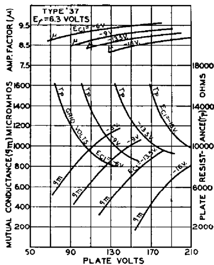
AVERAGE CHARACTERISTICS
