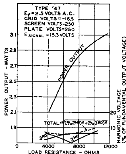
AVERAGE OUTPUT CHARACTERISTICS
