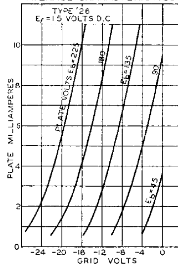
AVERAGE CHARACTERISTICS
