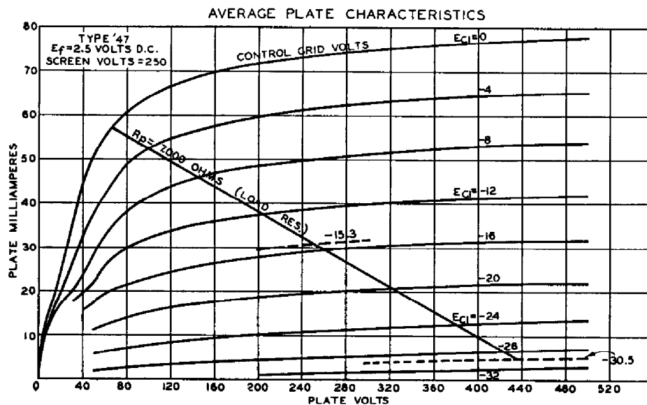
AVERAGE OUTPUT CHARACTERISTICS
