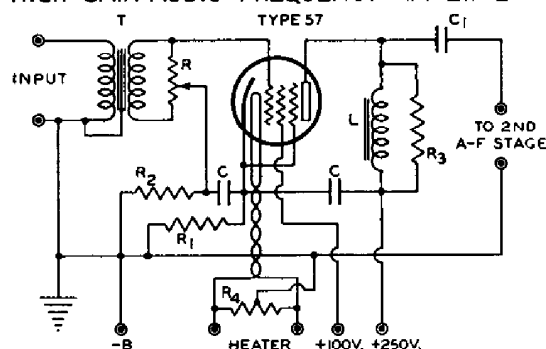
HIGH-GAIN AUDIO-FREQUENCY AMPLIFIER
