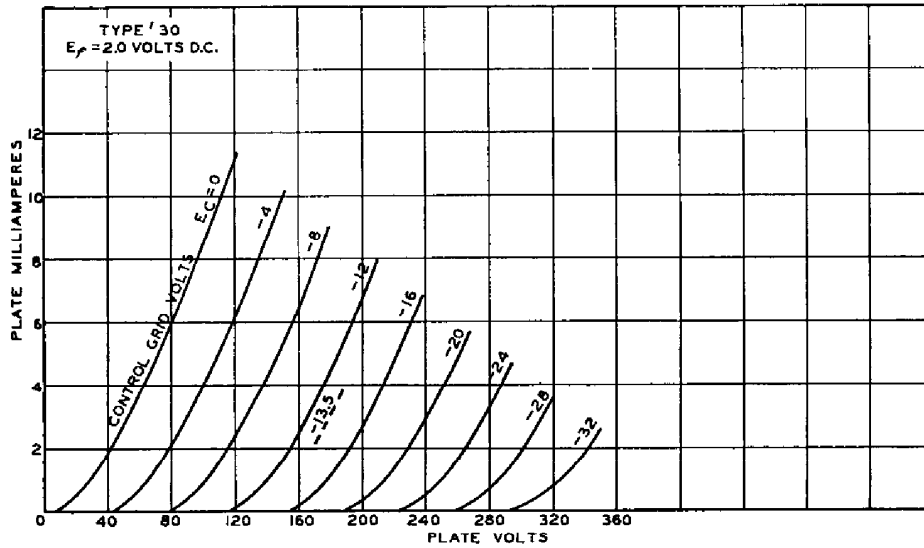
AVERAGE CHARACTERISTICS
